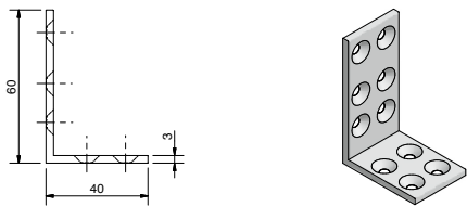
W36040...
