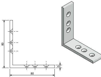
W58080...
