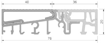
TSA5761/SK/EV1
