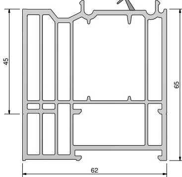
TSUK6265
