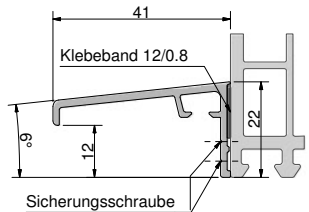
WS4125-6/SK/SF
