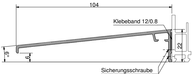
WS10422-6/SK/SF
