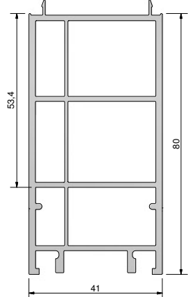
TSUK4180
