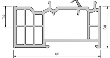
TSUK6230
