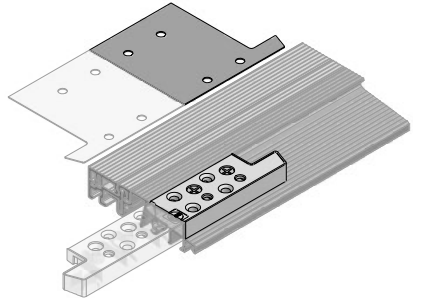
SH61-160g
